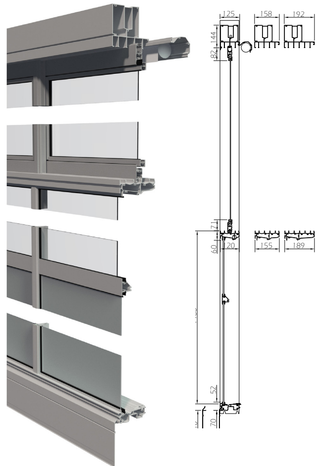
Twin Sight. Cross section and drawing from the side.
